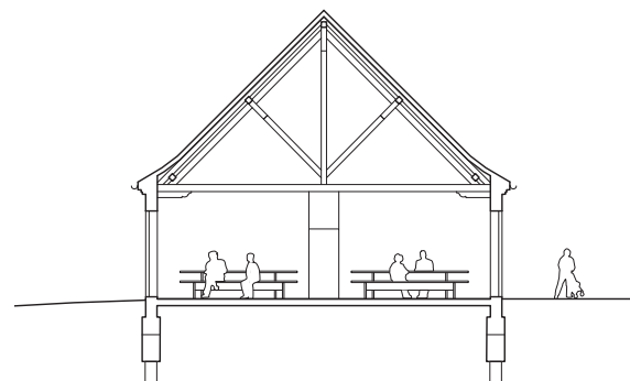
SNIT AA i Spisesal 1:250
